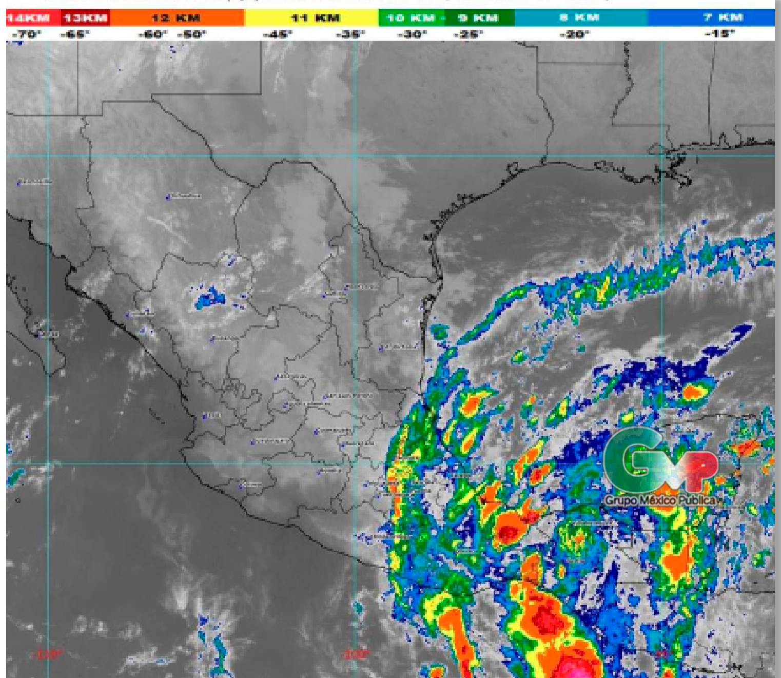
GOES-16 ABI Banda 13 Temp.[C] 20-Oct-2024 13:40:20 UTC (Local CDMX 07:40 Hrs.)
